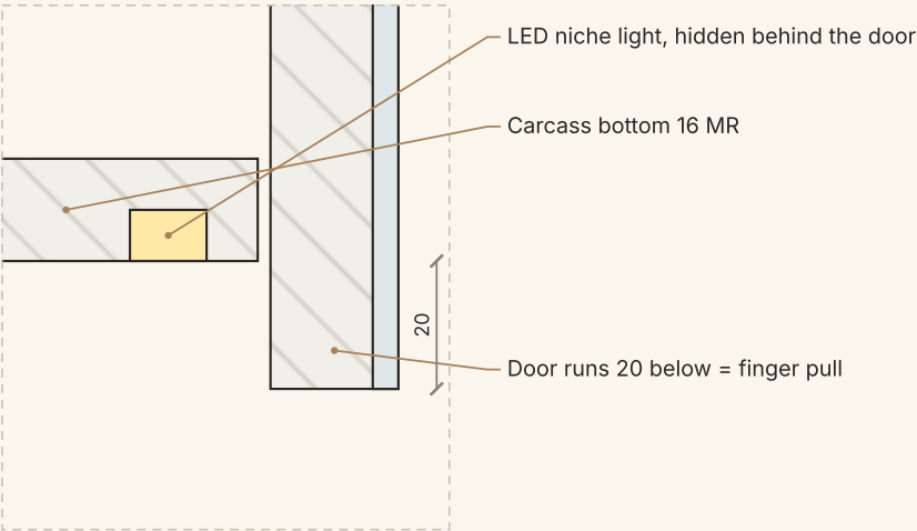
DETAIL C · FINGER PULL & NICHE LIGHT
