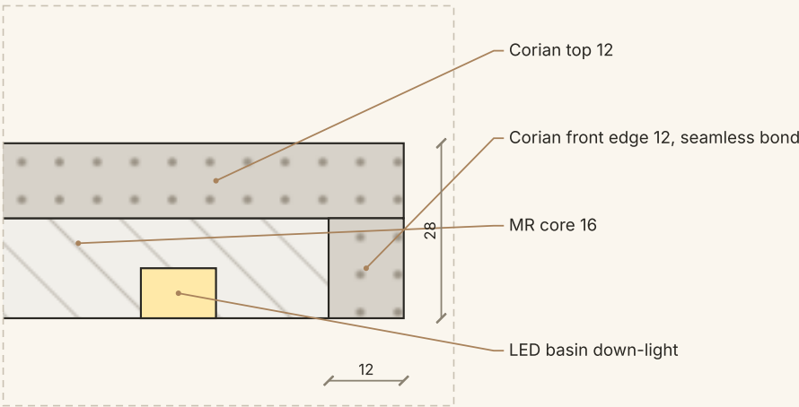
DETAIL D · CORIAN SHELF EDGE & BASIN LIGHT
