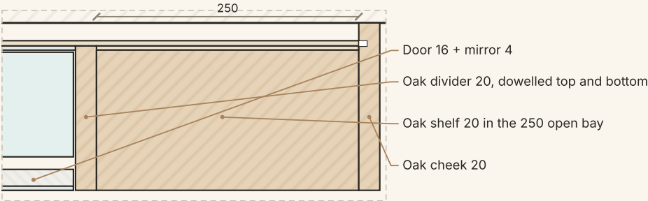
DETAIL E · PLAN: DOOR, DIVIDER & OPEN BAY
