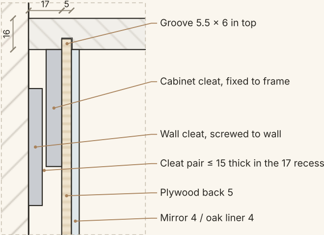
DETAIL B · BACK HOUSING & FRENCH CLEAT
