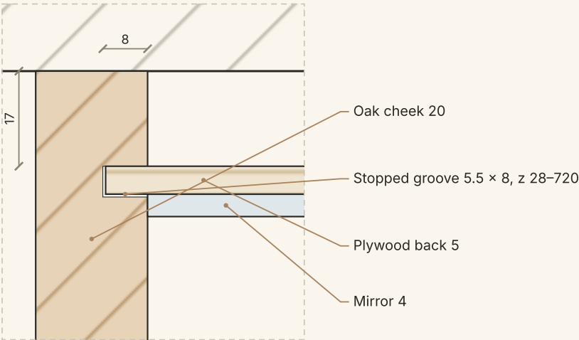
DETAIL E · PLAN, BACK IN CHEEK GROOVE
