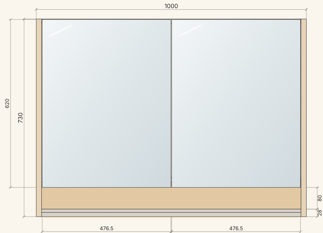
FRONT ELEVATION · SW-MC-100
