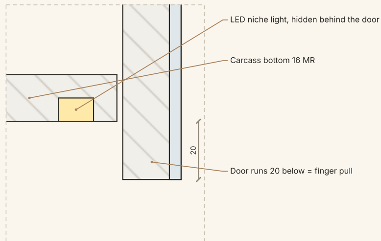
DETAIL C · FINGER PULL & NICHE LIGHT
