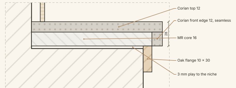
DETAIL D · CORIAN SHELF & BOTTOM FLANGE
