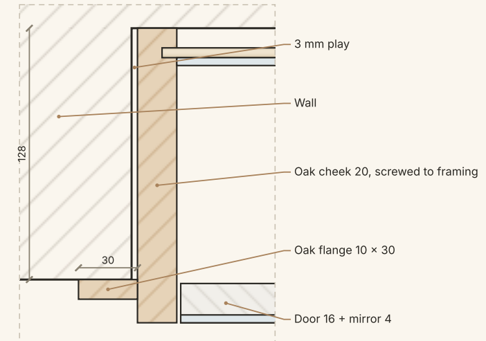
DETAIL E · PLAN: NICHE SIDE, FLANGE, CHEEK & DOOR
