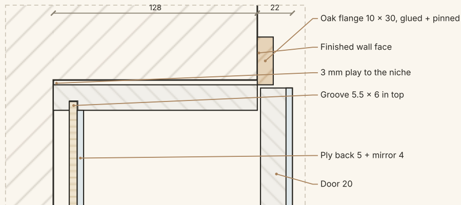
DETAIL B · TOP: NICHE, FLANGE & BACK
