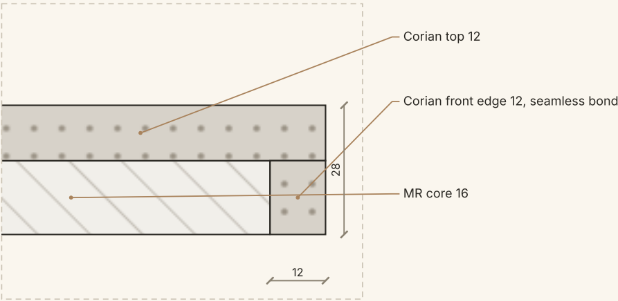
DETAIL D · 1400 VERSION: CORIAN NICHE SHELF
