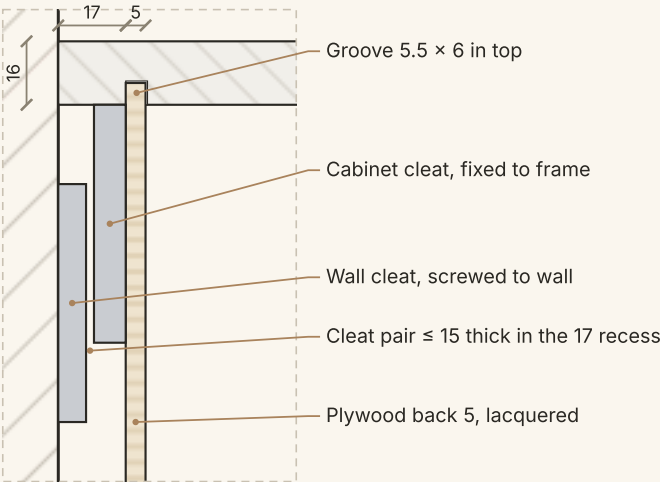
DETAIL B · BACK HOUSING & FRENCH CLEAT (ALL)
