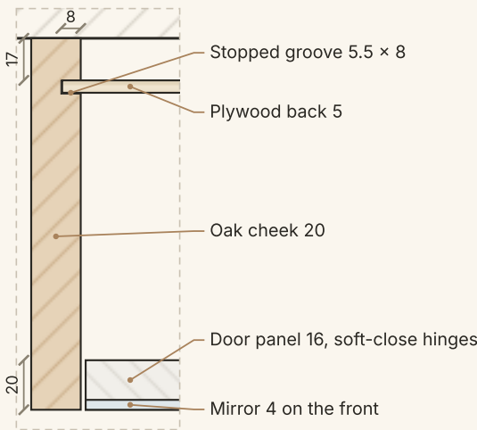
DETAIL E · PLAN, BACK IN CHEEK GROOVE & DOOR (15 DEEP)
