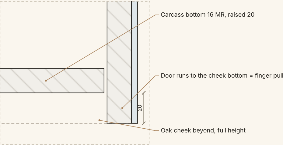
DETAIL C · 1200 VERSION: FINGER PULL AT THE BOTTOM
